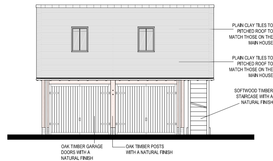
GARAGE FRONT ELEVATION - AS PROPOSED SCALE @ 1:100 ON AN A1 SHEET
