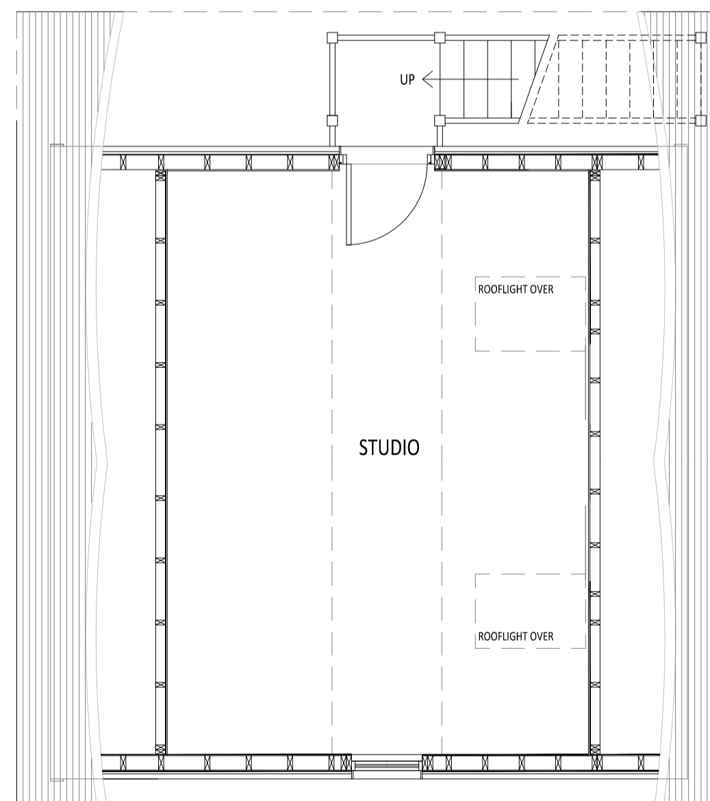
GARAGE FIRST FLOOR PLAN - AS PROPOSED SCALE @ 1:50 ON AN A1 SHEET
