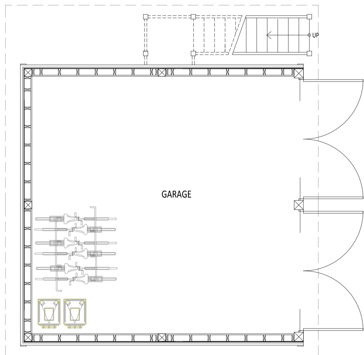
GARAGE GROUND FLOOR PLAN - AS PROPOSED SCALE @ 1:50 ON AN A1 SHEET
