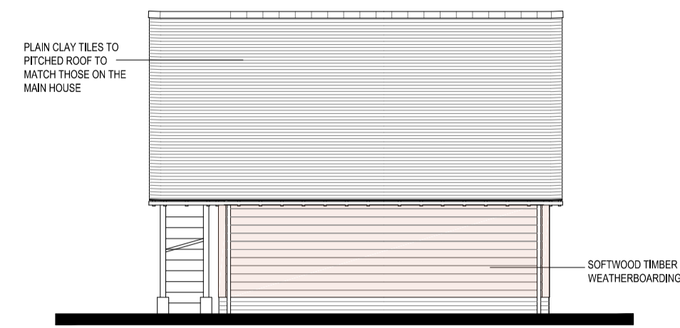
GARAGE REAR ELEVATION - AS PROPOSED SCALE @ 1:100 ON AN A1 SHEET
