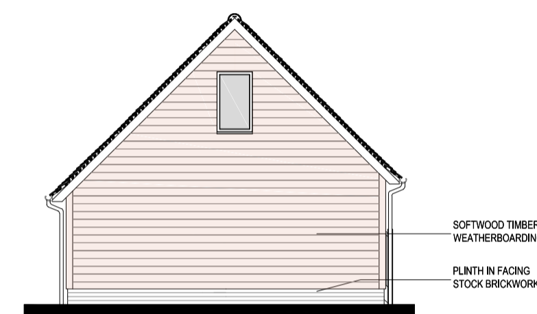
GARAGE SIDE (WEST) ELEVATION - AS PROPOSED SCALE @ 1:100 ON AN A1 SHEET
