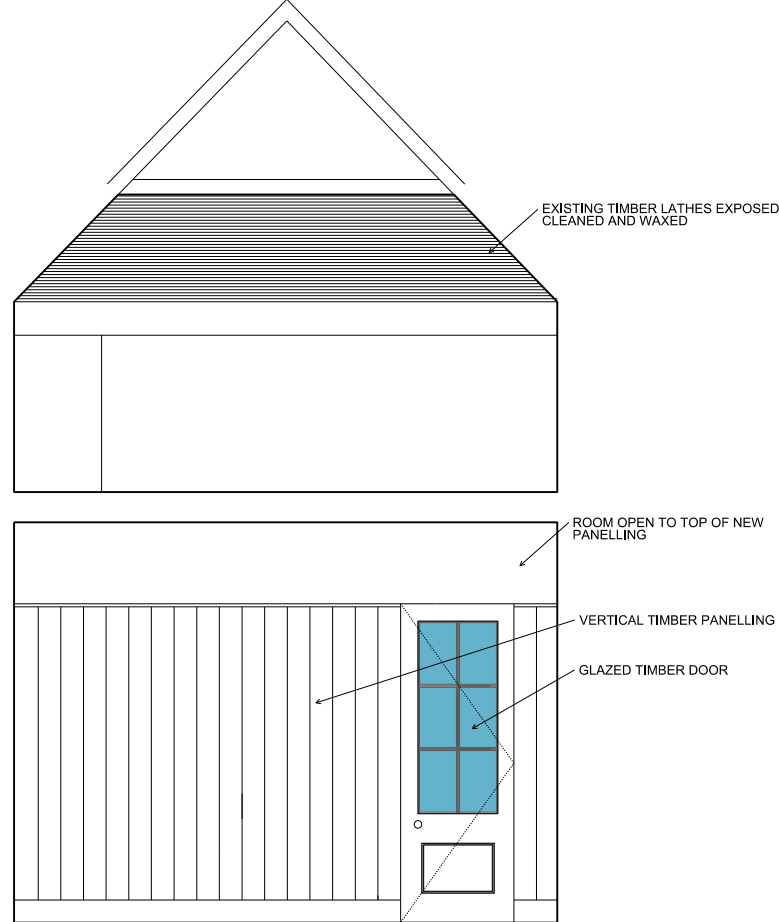
2 1:25 'RED HOUSE' INTERNAL ELEVATION
