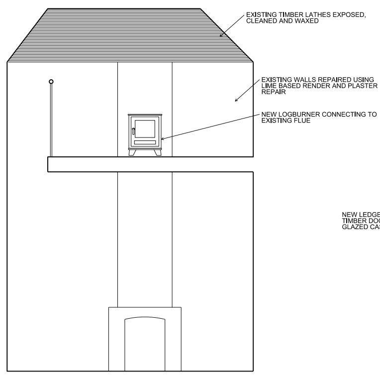
1 1:25 'RED HOUSE' INTERNAL ELEVATION
