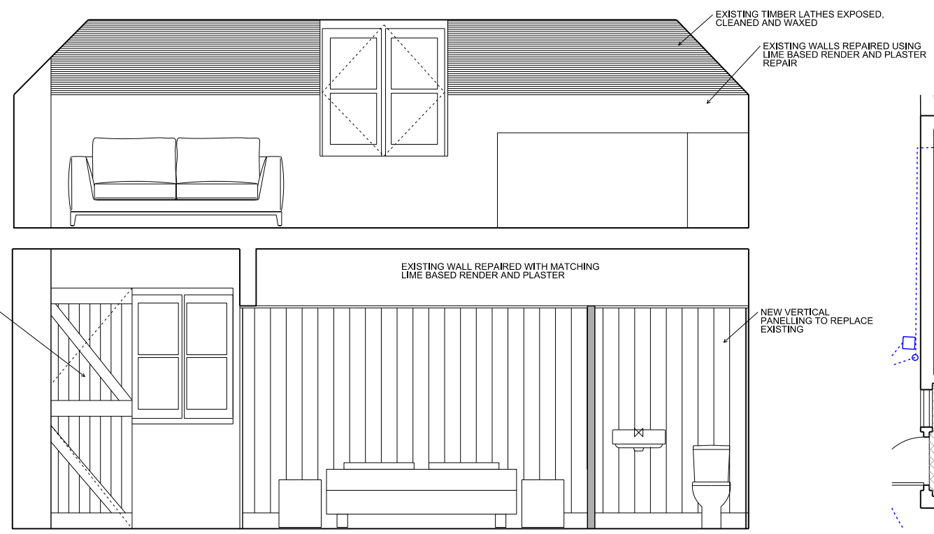
3 1:25 'RED HOUSE' INTERNAL ELEVATION
