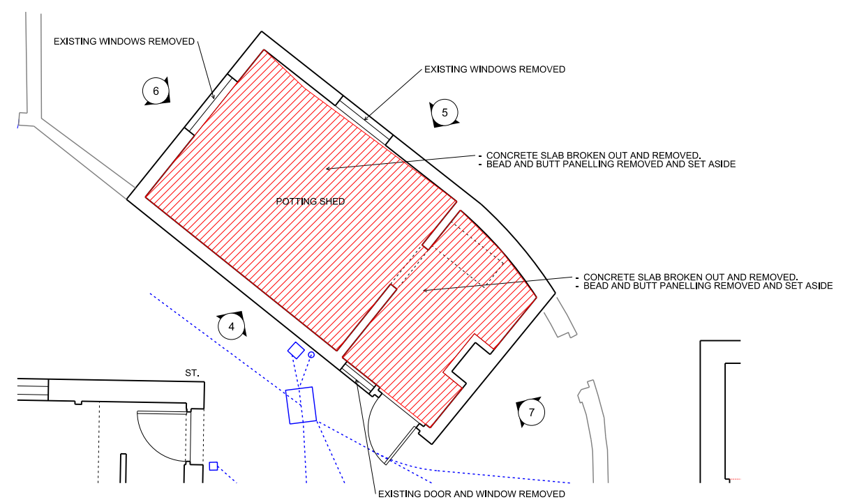
1 1:50 'RED HOUSE' GROUND PLAN
