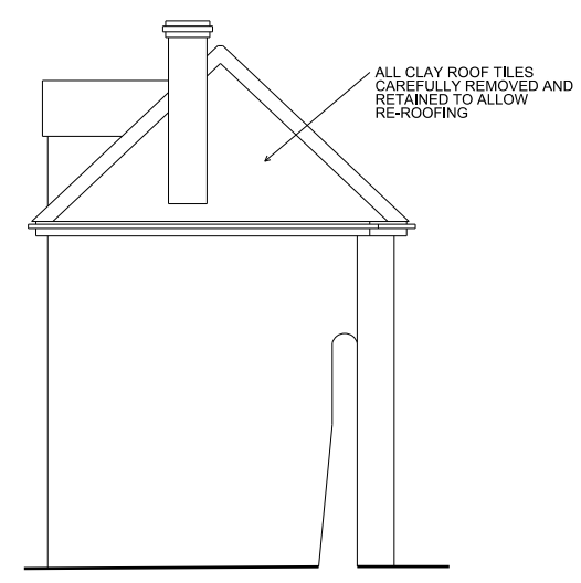
7 1:50 'RED HOUSE' EXISTING ELEVATION
