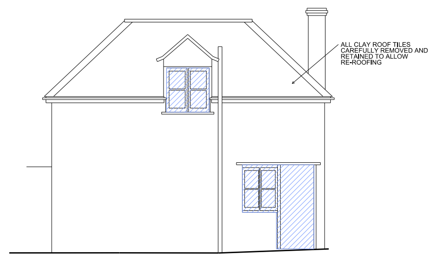
4 1:50 'RED HOUSE' EXISTING ELEVATION
