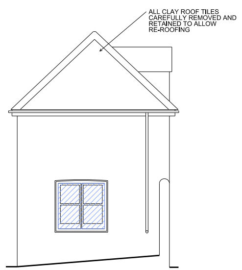
6 1:50 'RED HOUSE' EXISTING ELEVATION
