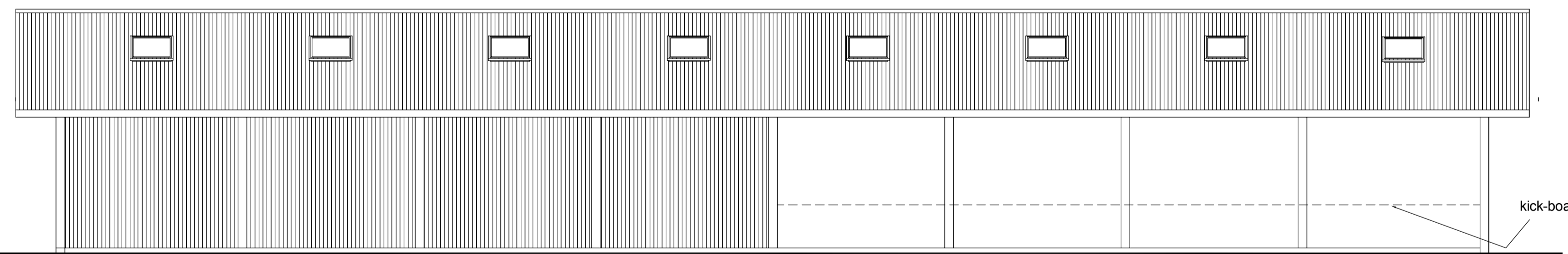
Side Elevation 2 (North West Face)
